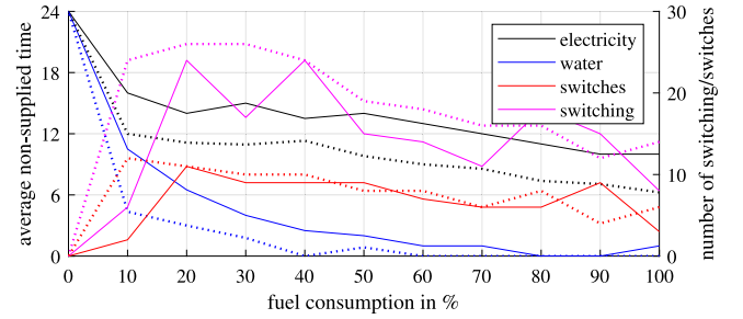
Fig. 4. Supply quality and number of switches for the 9-bus test example as a function of the fuel consumption L_g^{fuel} , (solid) even distribution considered ( \Pi_D = 1 ), (dashed) only average non-supply time minimized ( \Pi_D = 0 ).
