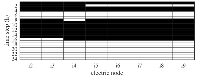
Fig. 3. The supply status (black is on) of the electric loads for the scenario shown in Fig. 2.
