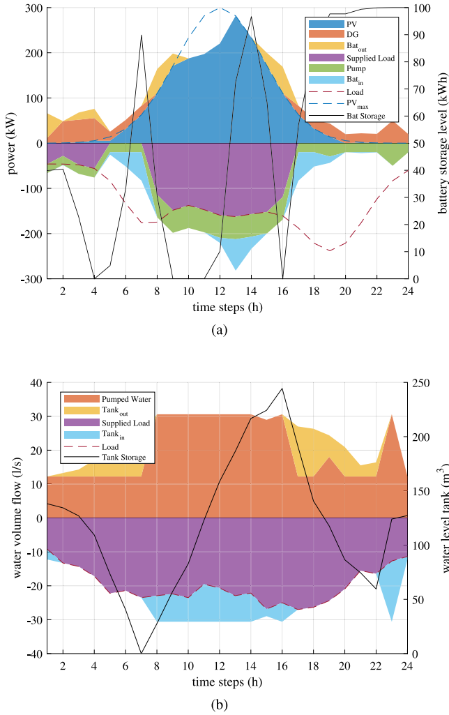
Fig. 2. Aggregated schedules for electricity (a) and for water (b) for one day of emergency operation of the 9-bus test network shown in Fig. 1.
